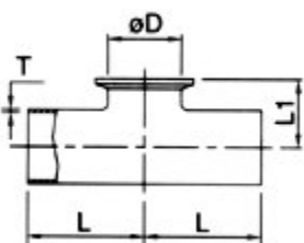
BPE Equal Outlet Tee Weld/ Clamp End (DT-15)
