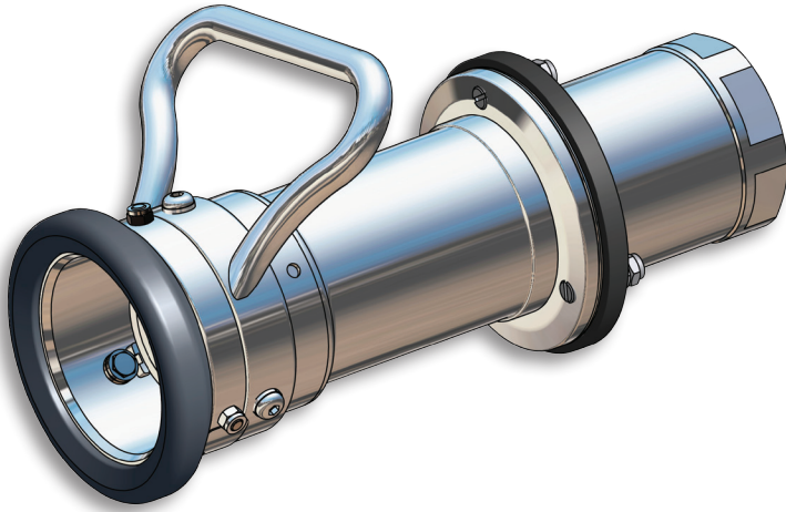
dry disconnect hose unit with break-away integrated
